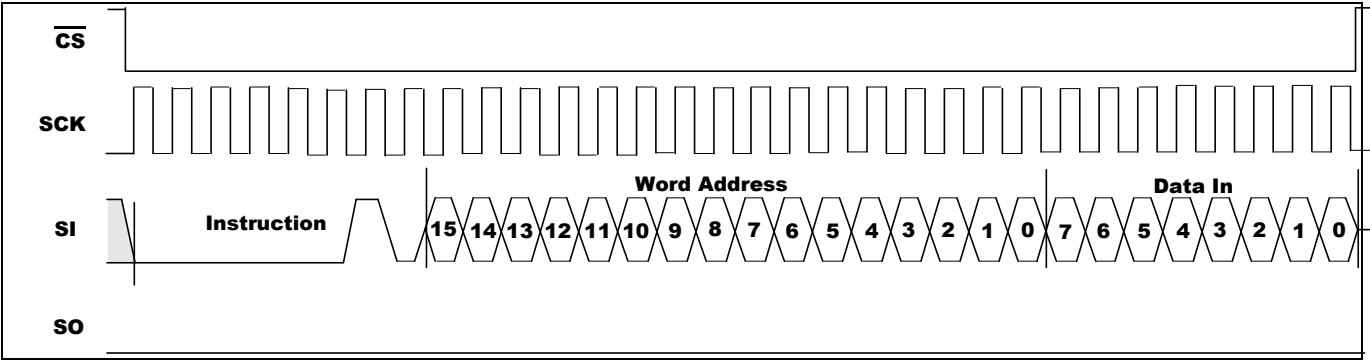
Figure 5-6. WRITE Sequence
