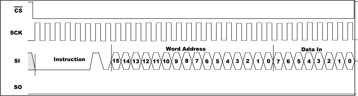
Figure 5-6. WRITE Sequence
