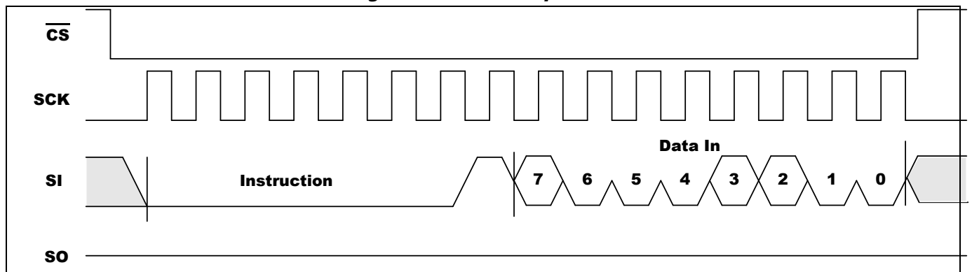
Figure 5-4. WRSR Sequence
