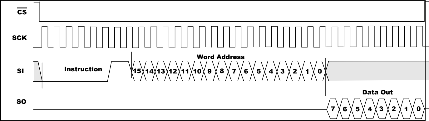
Figure 5-5. READ Sequence
