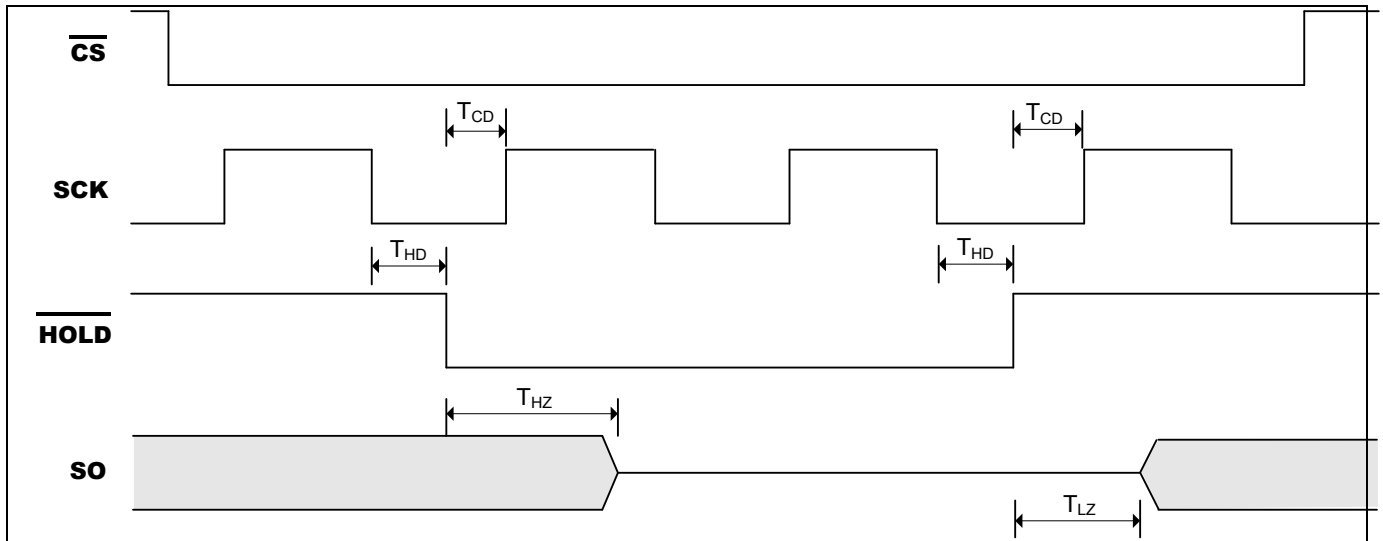
Figure 7-2. HOLD Timing
