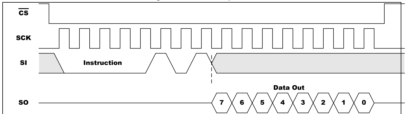
Figure 5-3. RDSR Sequence
